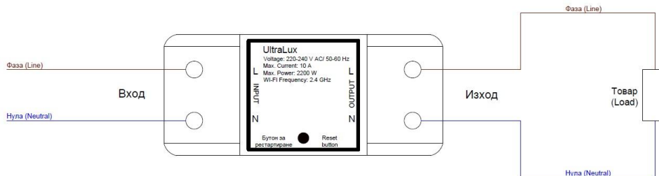
Connection diagram
